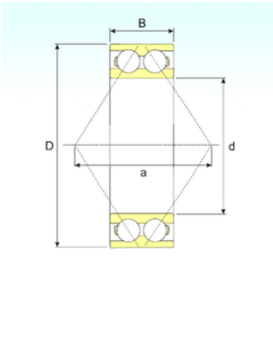
3204 A Bearing 2D drawings and 3D CAD models
