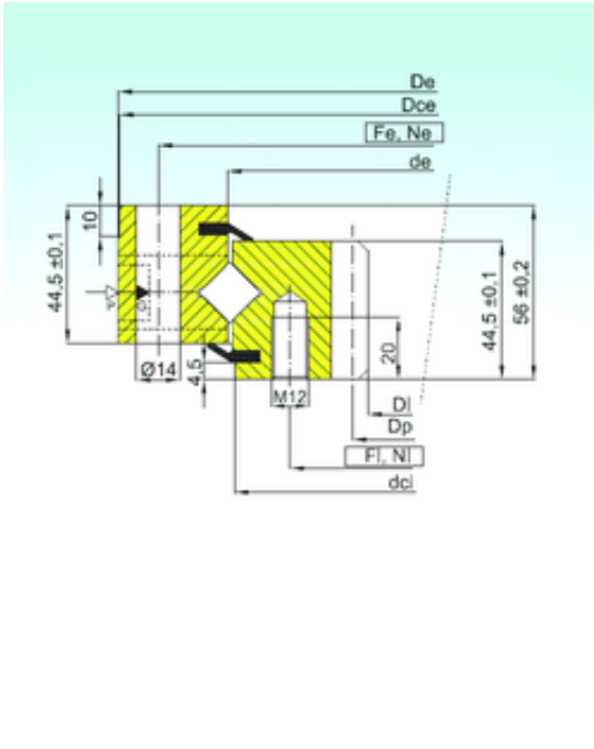
ZR1.14.0844.200-1SPTN Bearing 2D drawings and 3D CAD models
